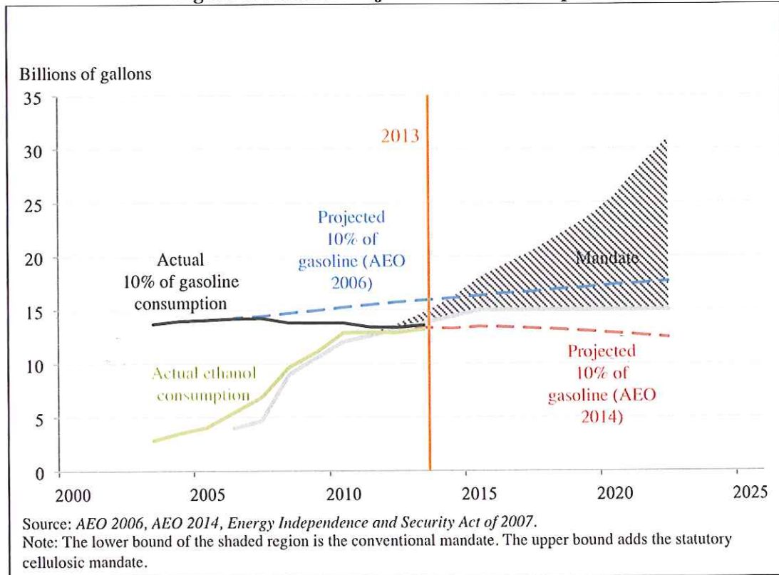
Figure 1: Ethanol Projection and Consumption
